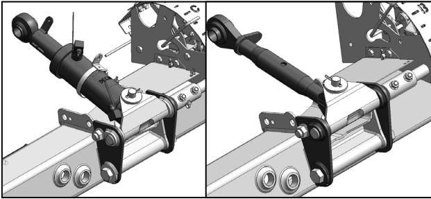
SHORT CENTER-LINK ASSEMBLIES
