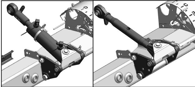
TYPICAL CENTER-LINK ASSEMBLIES
