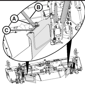
Side Deflectors
