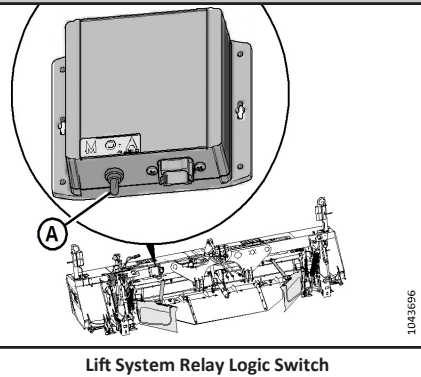
Lift System Relay Logic Switch
