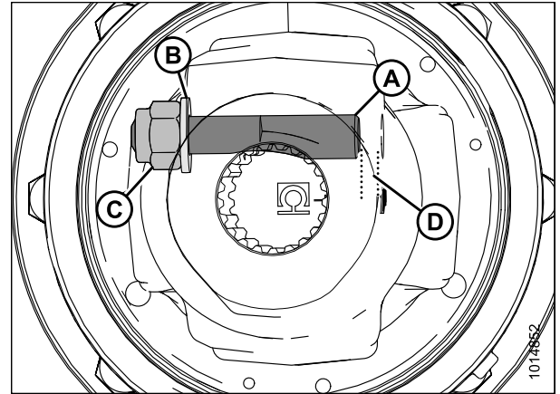
Figure 3.26: Transmission primaire
