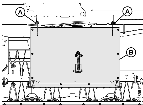
Figure 4.106: Blindage central
