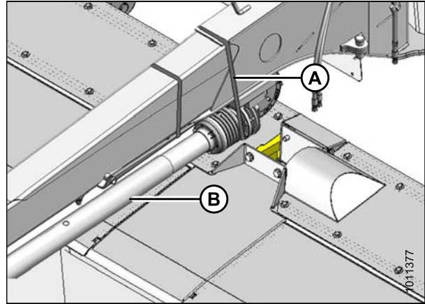
Figure 3.42: Cerclage de la transmission
