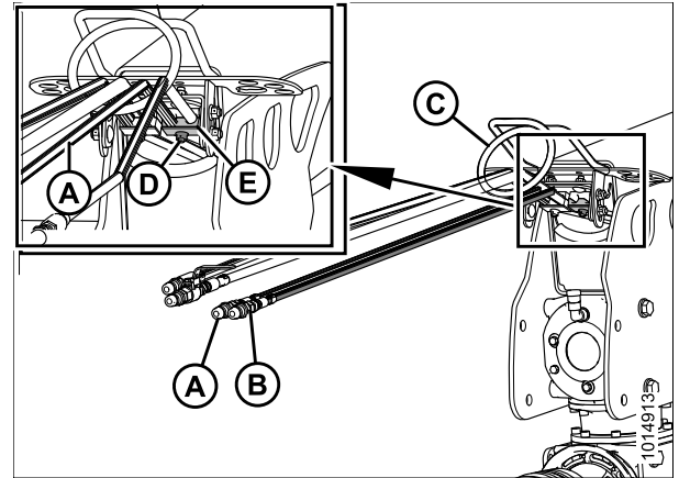
Figure 3.92: Flexibles de levage
