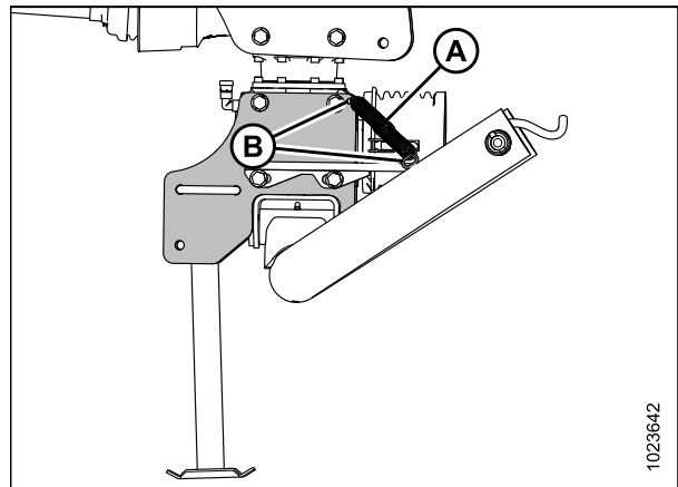
Figure 4.36: Ressorts
