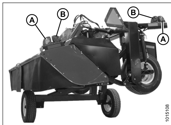
Figure 6.28: Road Friendly Transport™ (système de transport routier) Configuration
