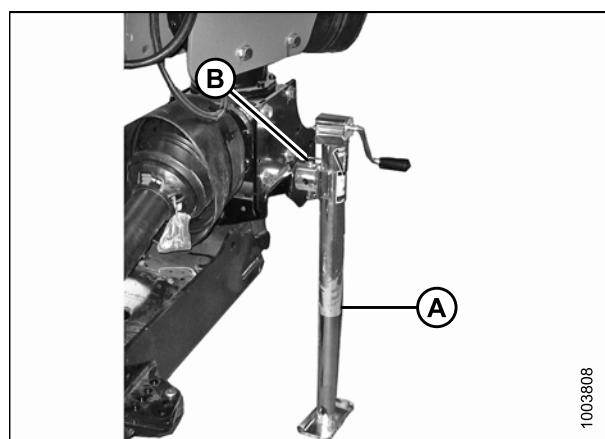
Figure 4.81: Cric d'attelage
