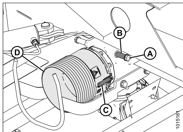
Figure 4.46: Blindage de la transmission
