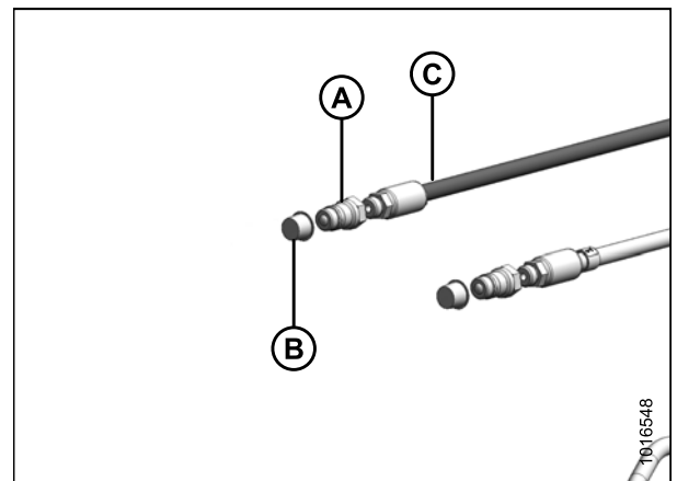
Figure 3.93: Raccords de flexible de levage
