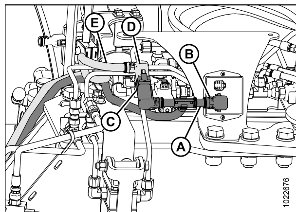
Figure 3.102: Raccordement du faisceau
