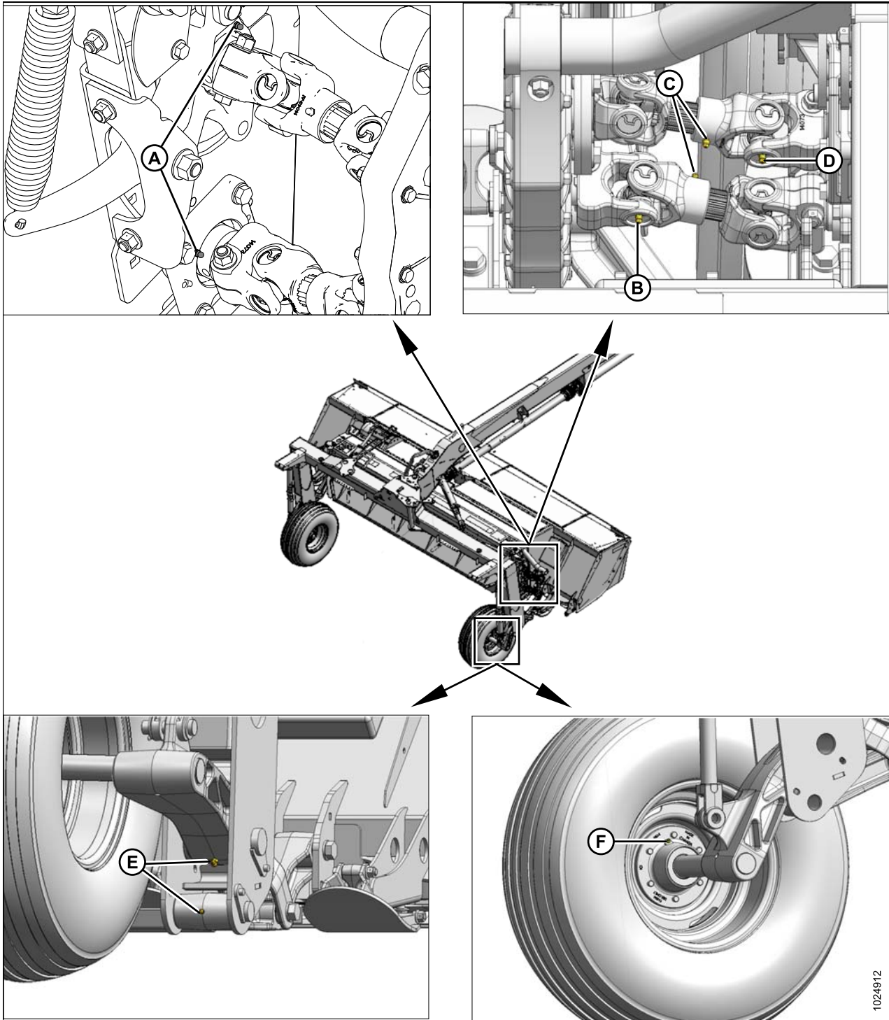
Figure 5.6: Points de lubrification
