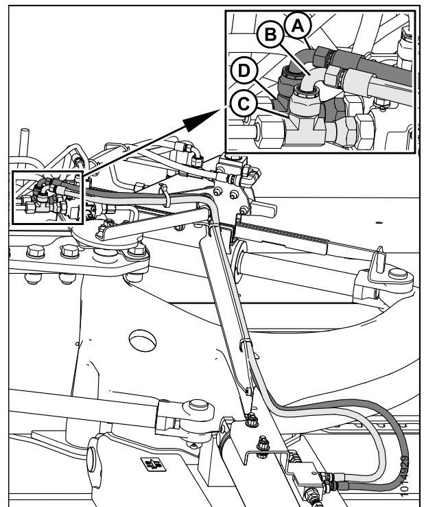
Figure 3.89: Commande de rotation de transport
