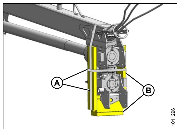
Figure 4.21: Emballage final de l'attelage
