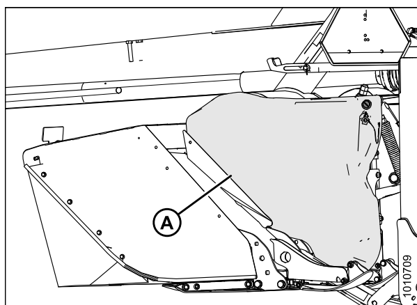
Figure 5.4: Blindage de la transmission
