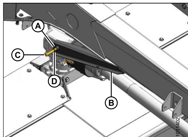
Figure 4.51: Bras de direction
