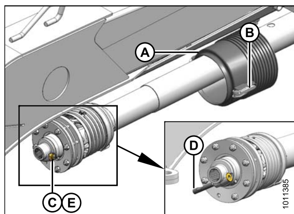
Figure 4.47: Transmission de l'embrayage
