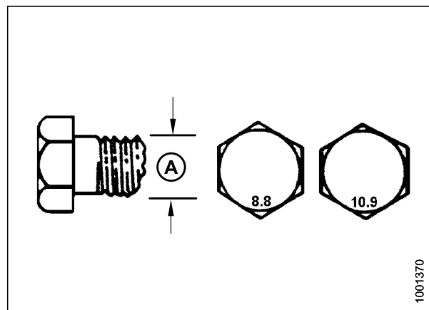
Figure 10.14: Grades des boulons
