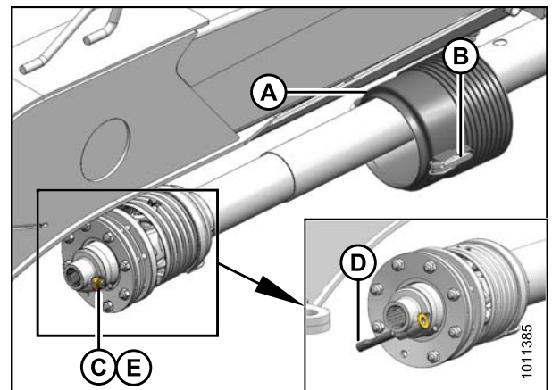
Figure 3.45: Transmission de l'embrayage
