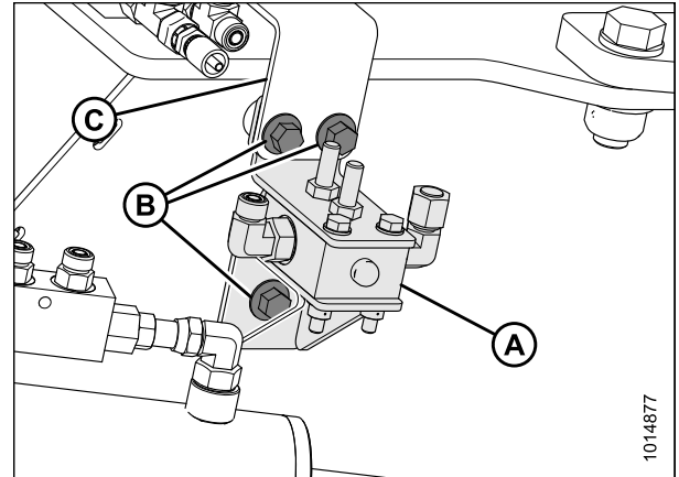
Figure 3.83: Vanne de commande
