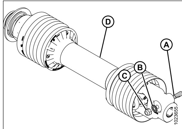
Figure 3.35: Transmission primaire
