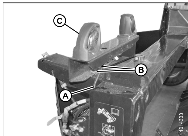
Figure 3.53: Support du feu
