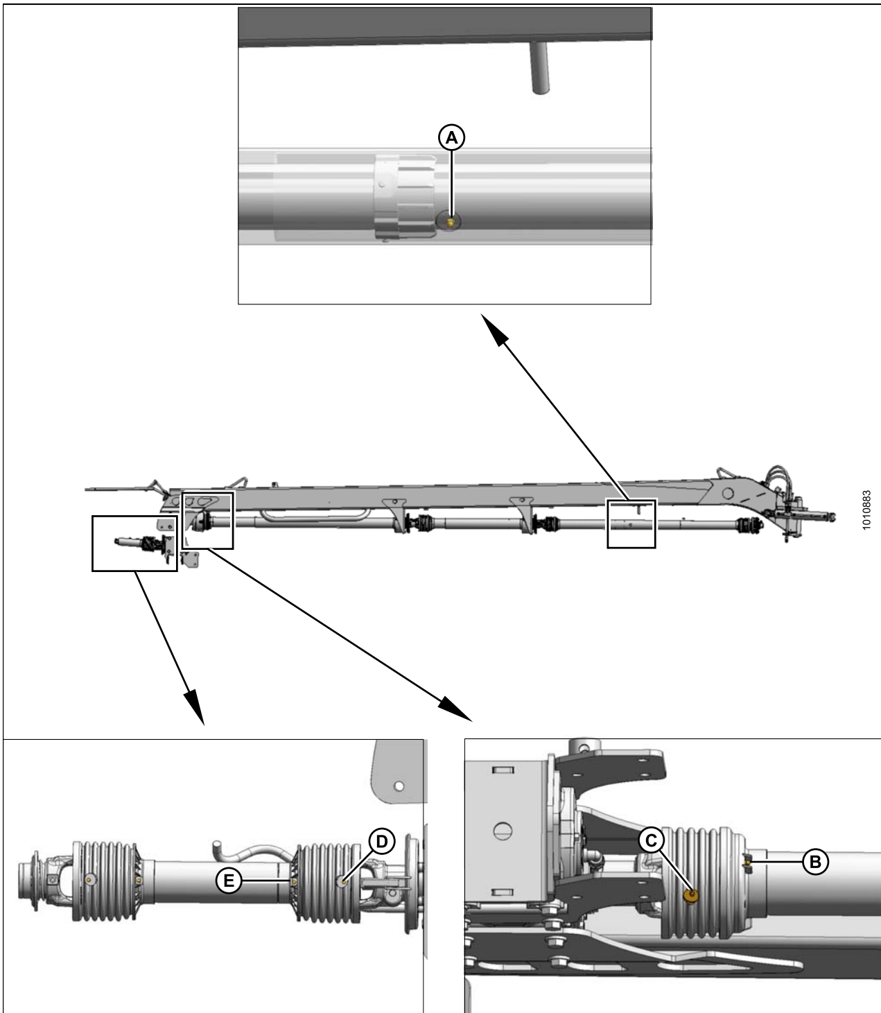
Figure 5.8: Points de lubrification
