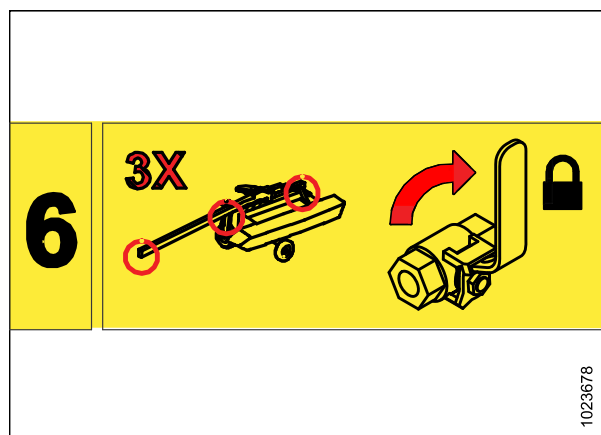
Figure 6.48: Verrouillage hydraulique
