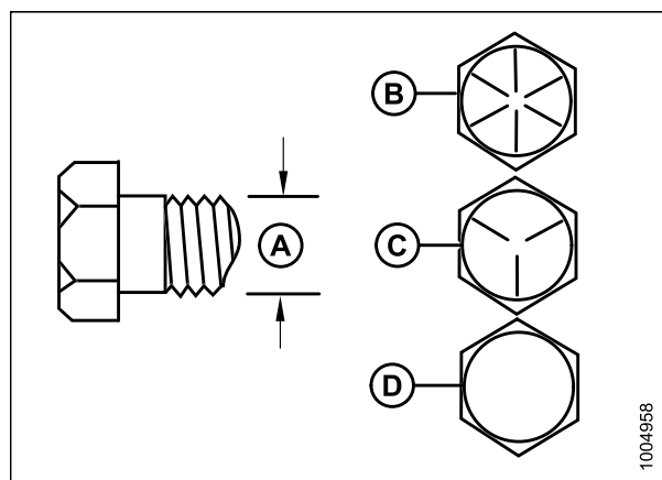
Figure 10.8: Grades des boulons
