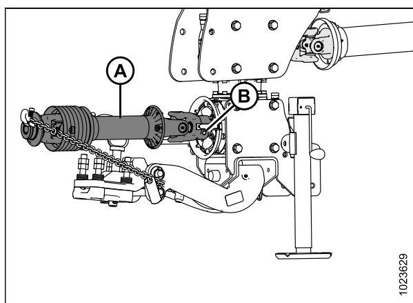
Figure 3.25: Transmission primaire
