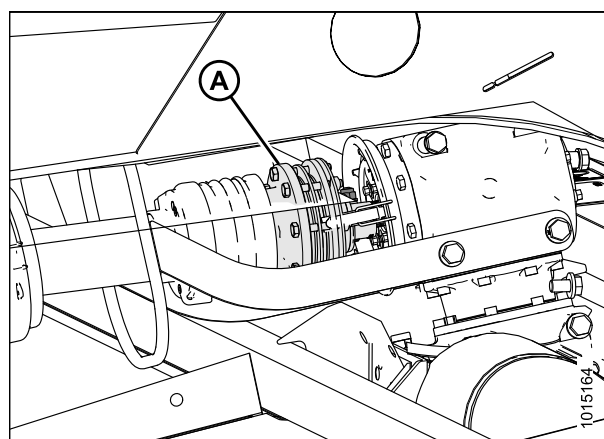
Figure 4.48: Transmission de l'embrayage
