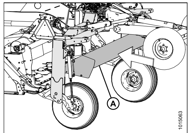
Figure 3.164: Blindage tourné
