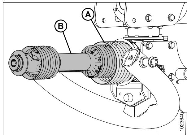
Figure 3.38: Protection conique
