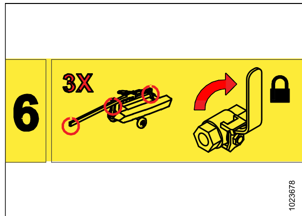
Figure 7.22: Verrouillage hydraulique
