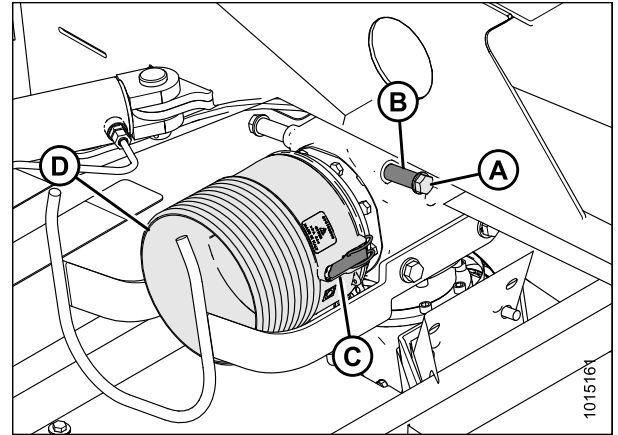
Figure 3.44: Blindage de la transmission
