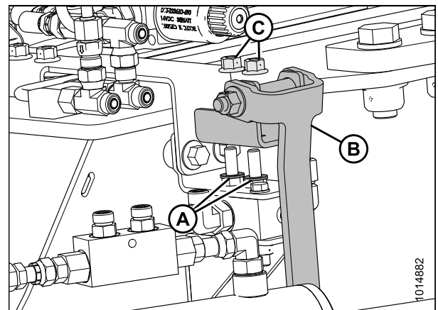
Figure 3.84: Vanne de commande
