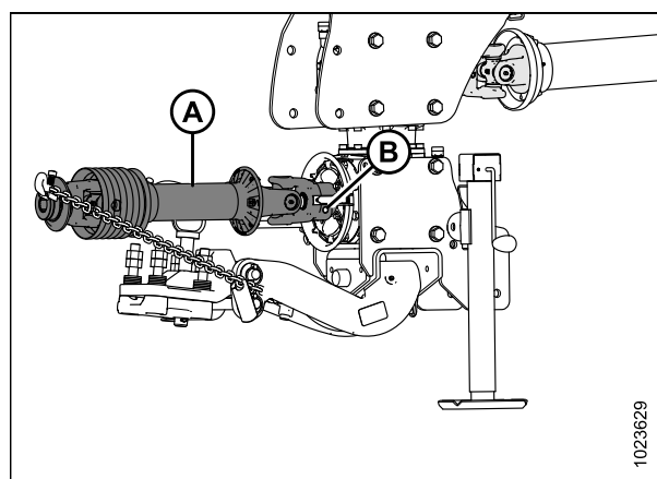
Figure 4.28: Transmission primaire
