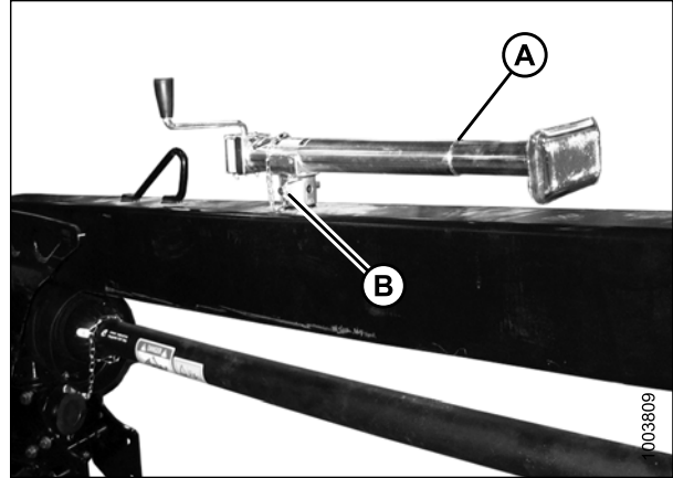
Figure 3.120: Rangement du cric
