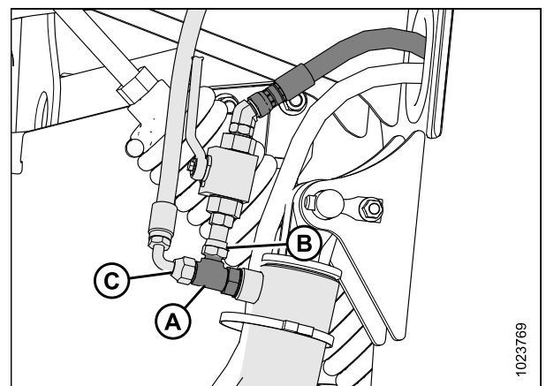
Figure 3.56: Tuyauterie du loquet
