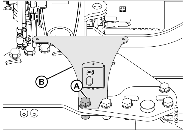
Figure 3.63: Support de capot
