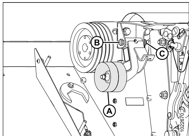
Figure 8.25: Tendeur
