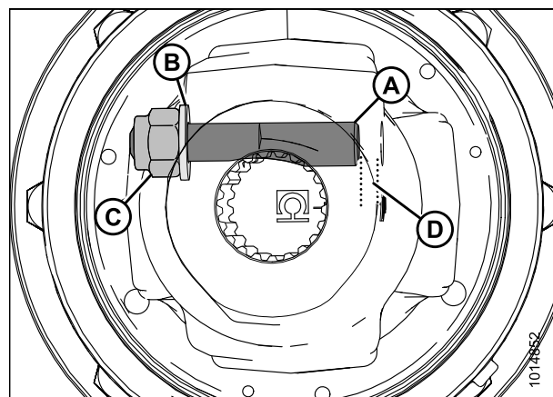
Figure 3.37: Transmission primaire
