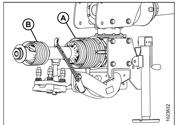
Figure 3.27: Protection conique
