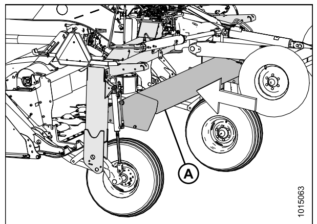
Figure 4.130: Blindage tourné
