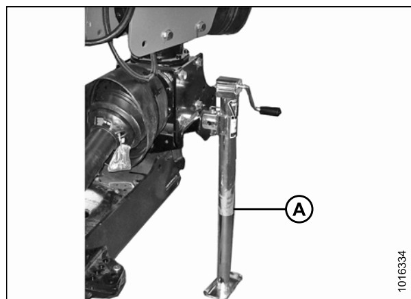
Figure 6.13: Cric d'attelage
