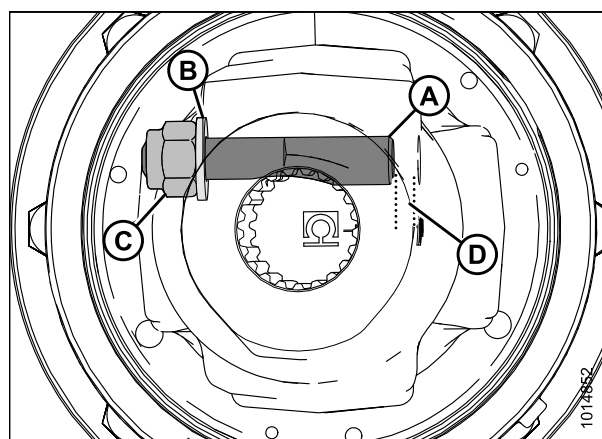
Figure 4.40: Transmission primaire
