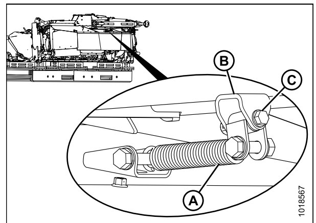
Figure 3.142: Ressort fixé au transport
