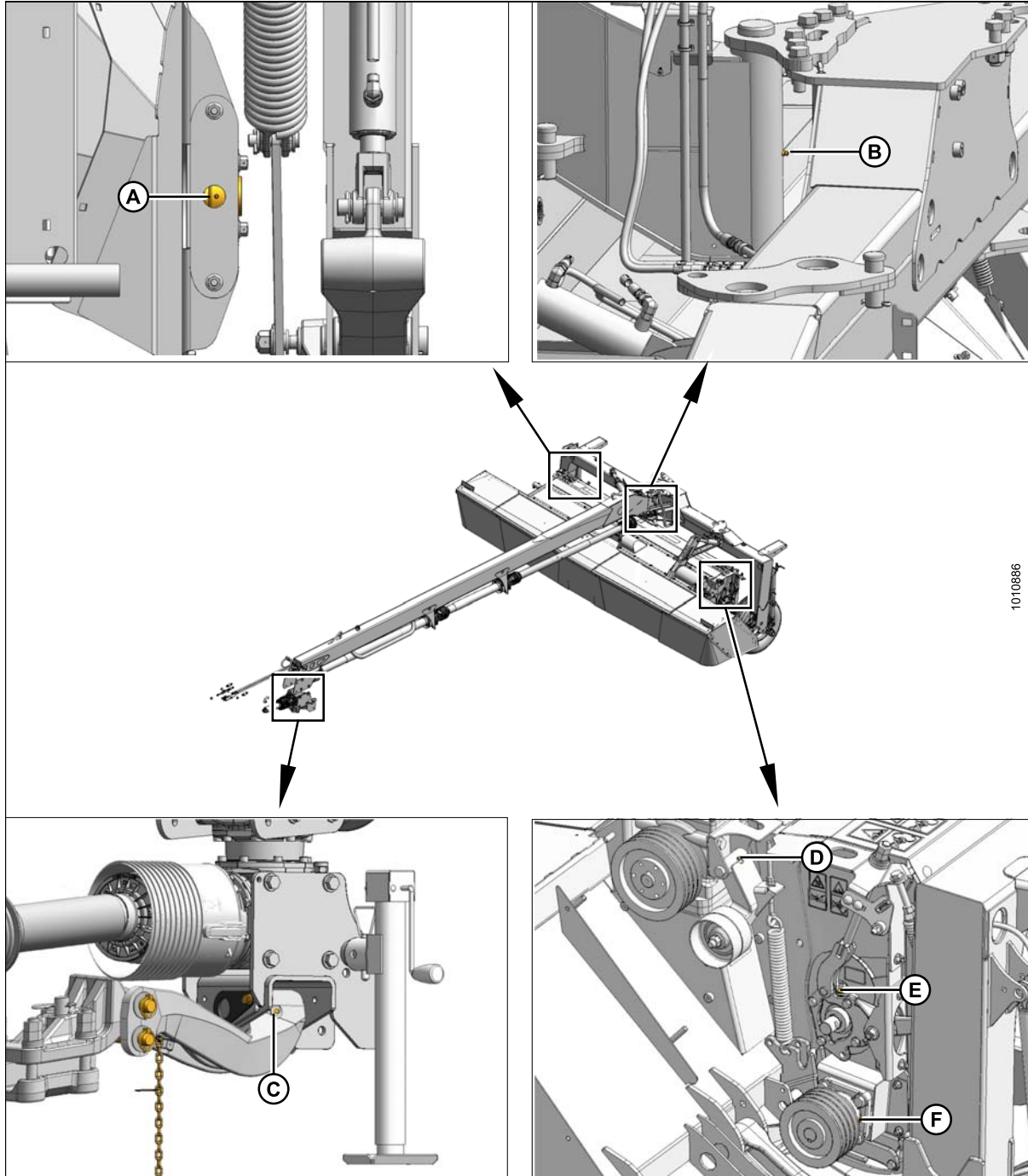
Figure 5.5: Points de lubrification
