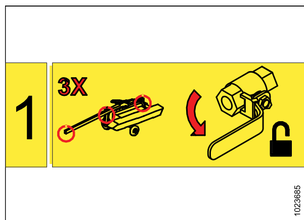
Figure 6.55: Verrouillage hydraulique
