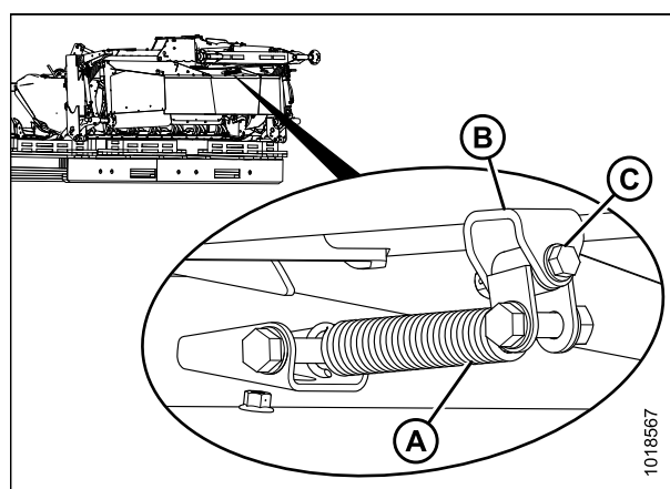
Figure 4.109: Ressort fixé au transport
