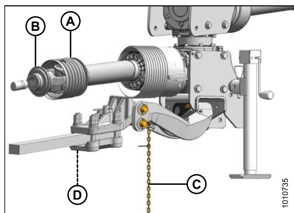
Figure 4.80: Transmission primaire
