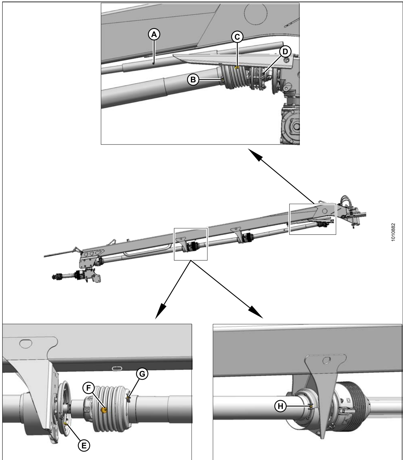
Figure 5.9: Points de lubrification
