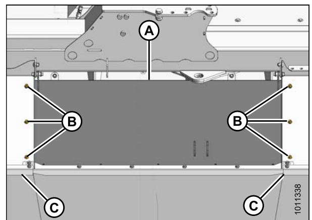
Figure 3.143: Ensemble du capot central
