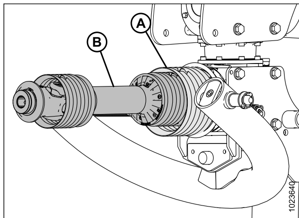
Figure 4.41: Protection conique
