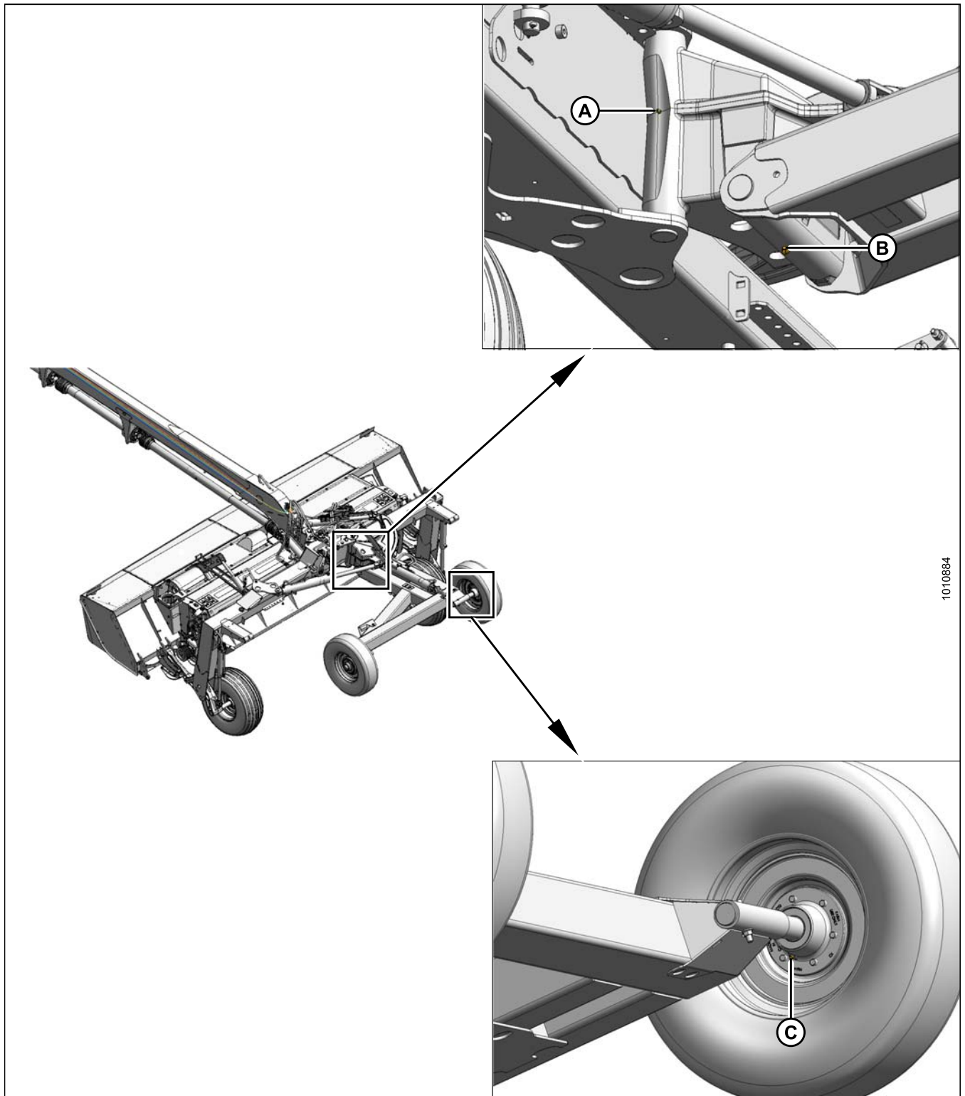
Figure 5.7: Points de lubrification
