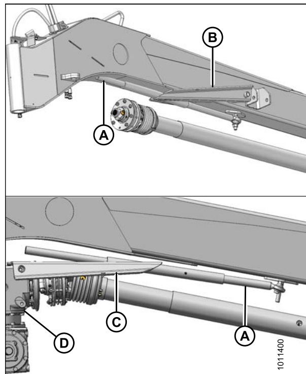
Figure 4.50: Bras de direction
