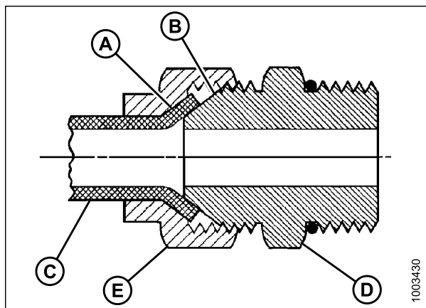
Figure 10.15: Raccord hydraulique
