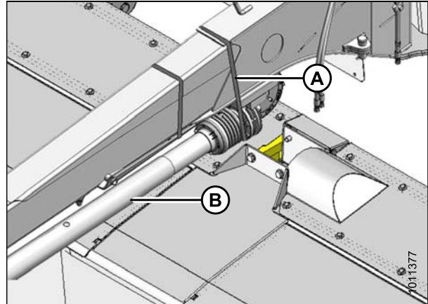
Figure 4.44: Cerclage de la transmission
