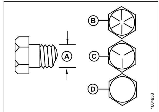
Figure 10.6: Grades des boulons
