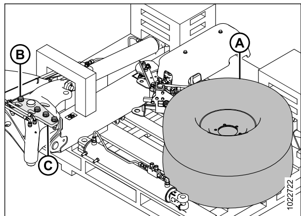
Figure 3.59: Emballage du transport
