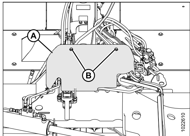
Figure 3.112: Capot
