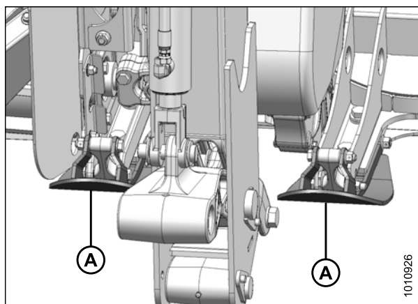
Figure 6.8: Patins 4,9 m (16 pi)
