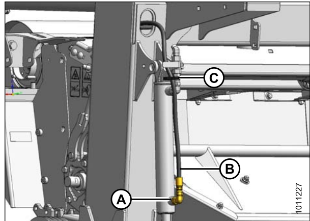
Figure 3.96: Vérin de levage
