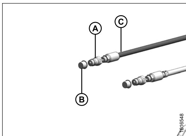
Figure 4.64: Raccords de flexible de levage
