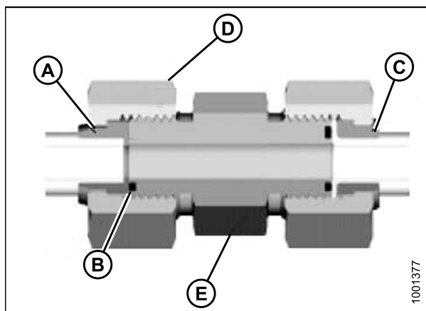
Figure 10.20: Raccord hydraulique
