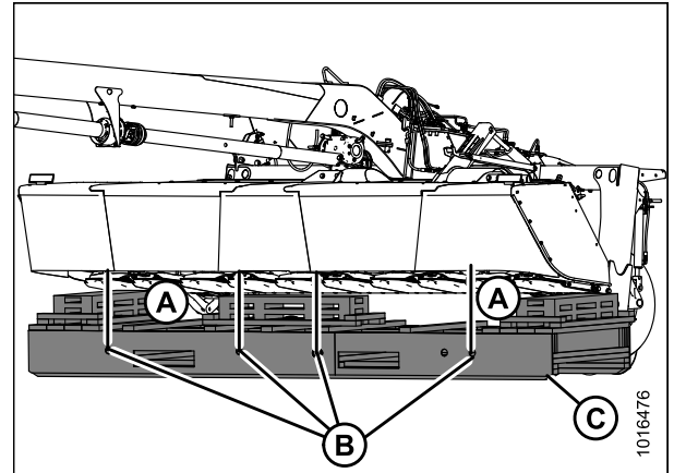
Figure 3.168: Cerclage
