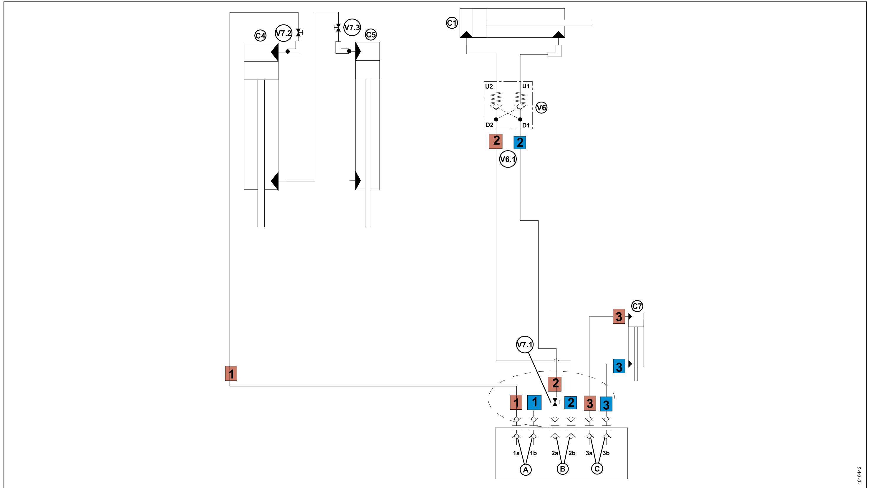
Figure 9.2: Schéma hydraulique – sans transport
