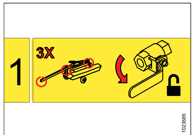
Figure 7.29: Verrouillage hydraulique
