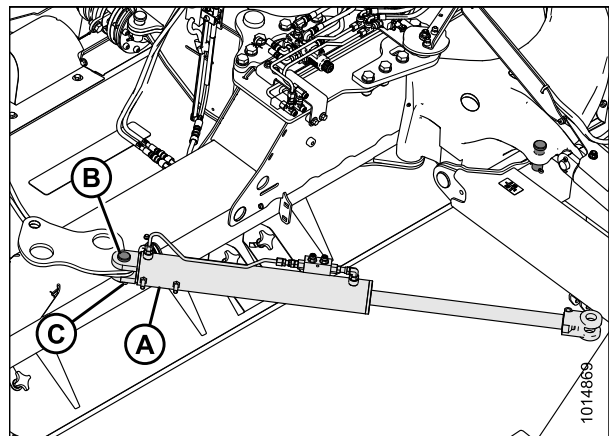
Figure 3.71: Vérin de rotation de transport
