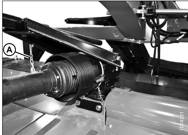
Figure 3.50: Blindage de la transmission
