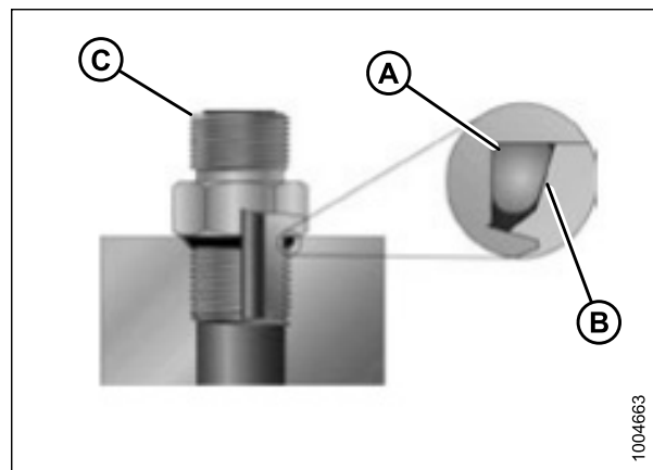
Figure 10.18: Raccord hydraulique
