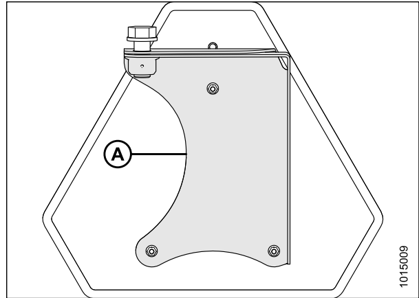
Figure 3.110: Panneau VLM
