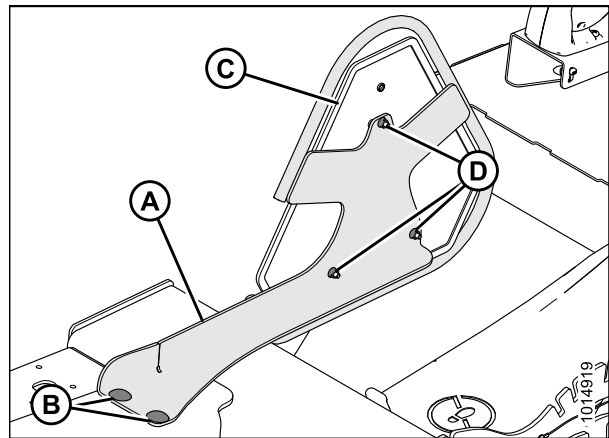
Figure 3.111: Panneau VLM
