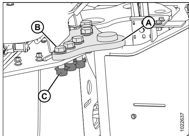
Figure 4.20: Broche du pivot
