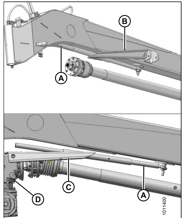
Figure 3.48: Bras de direction
