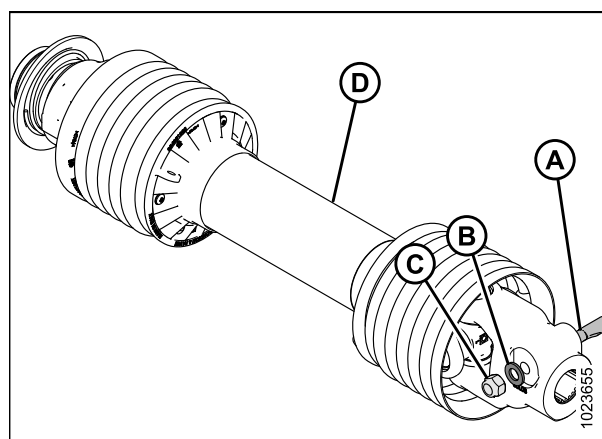
Figure 4.27: Transmission primaire
