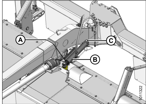
Figure 3.39: Vérin de direction
