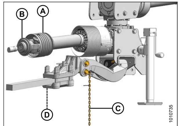
Figure 3.118: Transmission primaire
