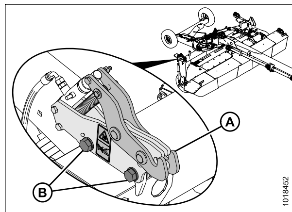
Figure 6.41: Loquet de transport
