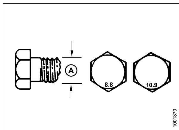
Figure 10.12: Grades des boulons
