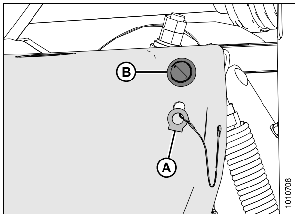
Figure 5.3: Loquet du blindage de la transmission
