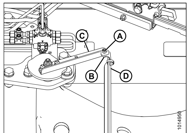
Figure 3.68: Plaque de support
