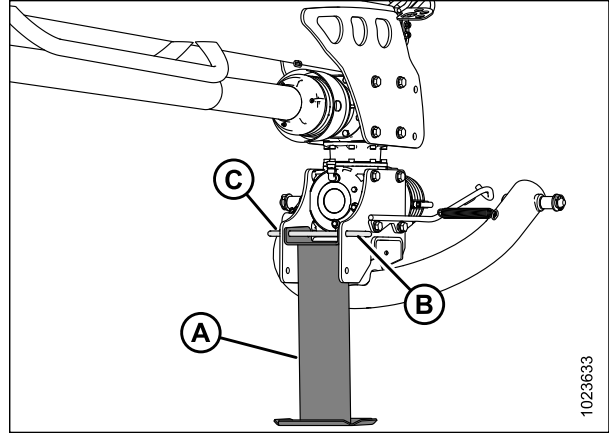
Figure 4.35: Chandelle
