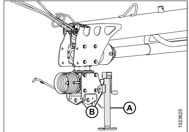
Figure 3.20: Attelage
