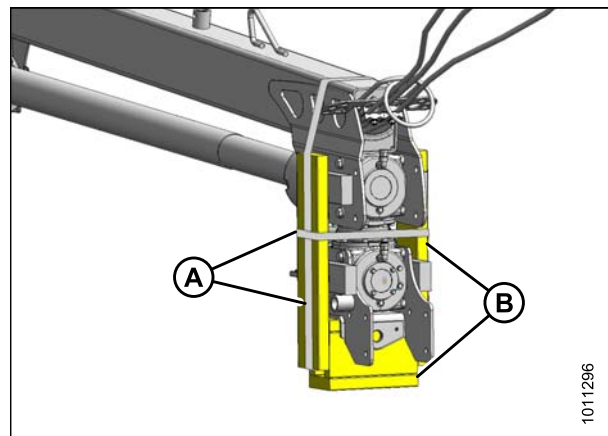
Figure 3.18: Emballage final de l'attelage
