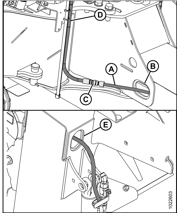
Figure 3.95: Flexible de levage
