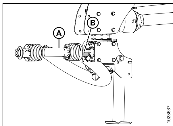
Figure 4.39: Transmission primaire
