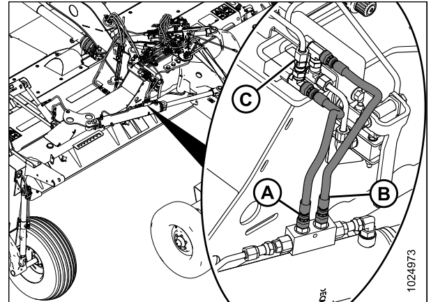
Figure 3.88: Vérin de rotation de transport
