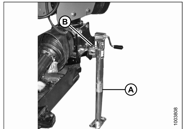
Figure 3.119: Cric d'attelage
