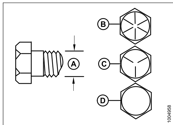
Figure 10.9: Grades des boulons
