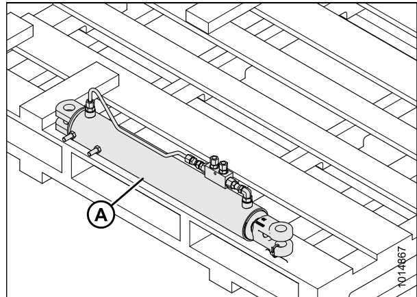
Figure 3.69: Vérin de rotation de transport
