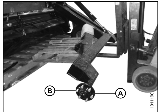
Figure 3.73: Roue de transport
