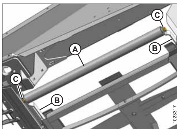
Figura 5.253: Rodillo tensor
