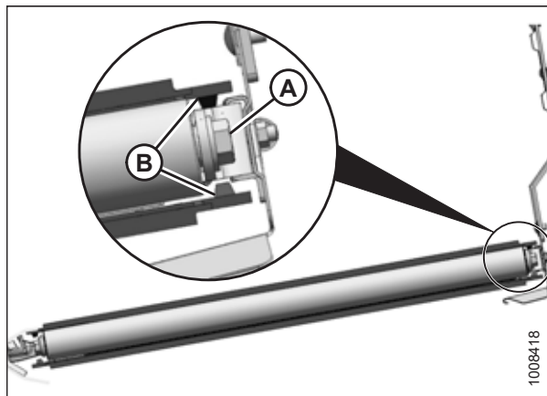
Figura 5.240: Rodillo tensor
