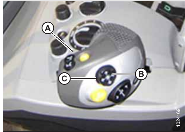
Figura 3.117: Joystick CLAAS 600/700
