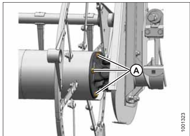
Figura 5.371: Cruceta
