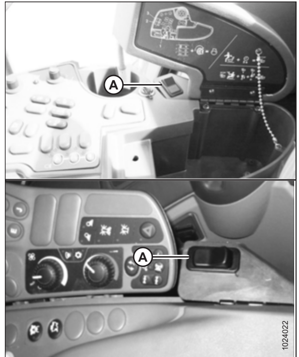
Figura 3.120: Consolas John Deere
