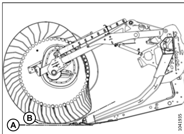
Figure 3.60: Profil des doigts – Position 2 de la came
