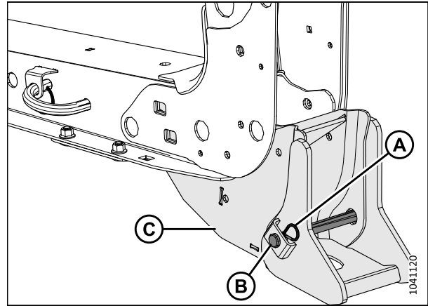
Figure 4.123: Support de la plateforme
