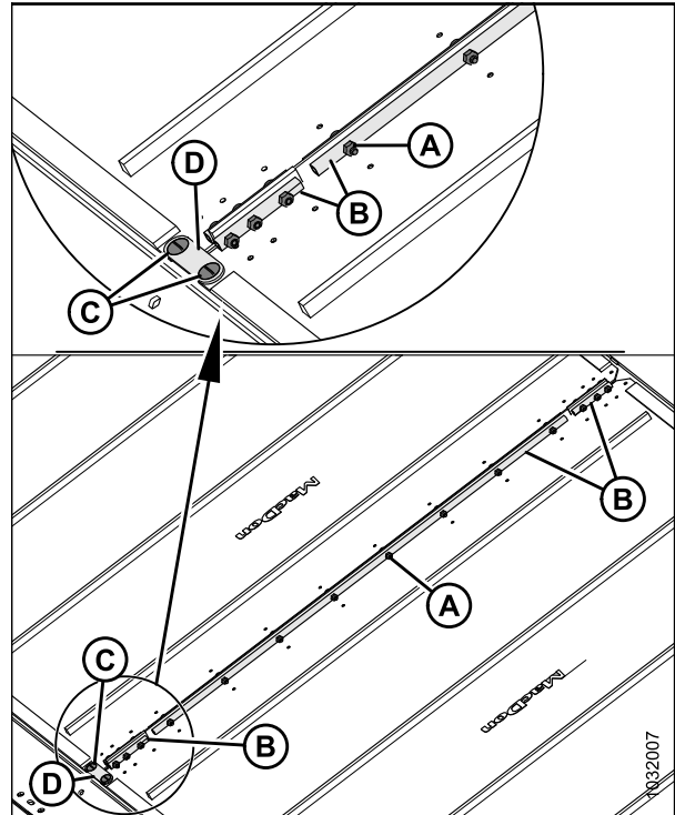
Figure 5.91: Raccordements du tapis
