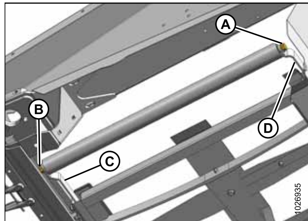
Figure 5.104: Rouleau libre
