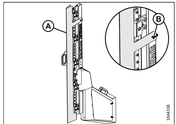
Figure 5.236: Couteau vertical
