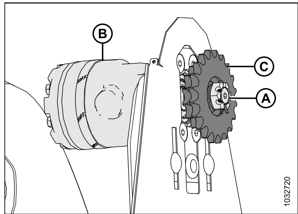
Figure 5.218: Pignon double
