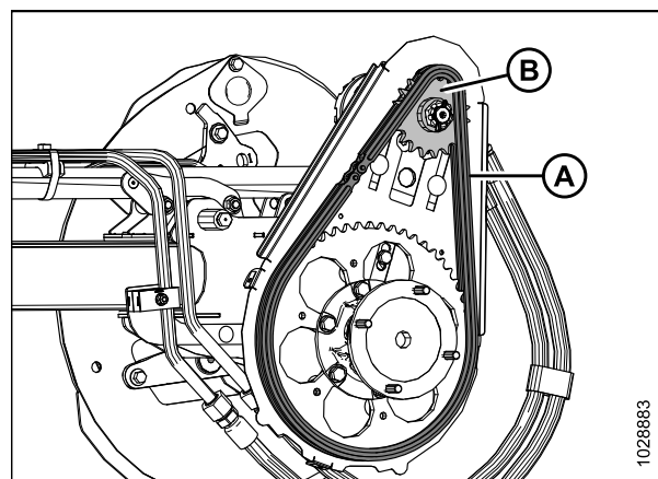
Figure 5.212: Pignon unique
