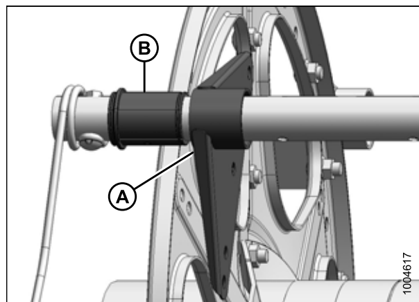
Figure 5.154: Bague
