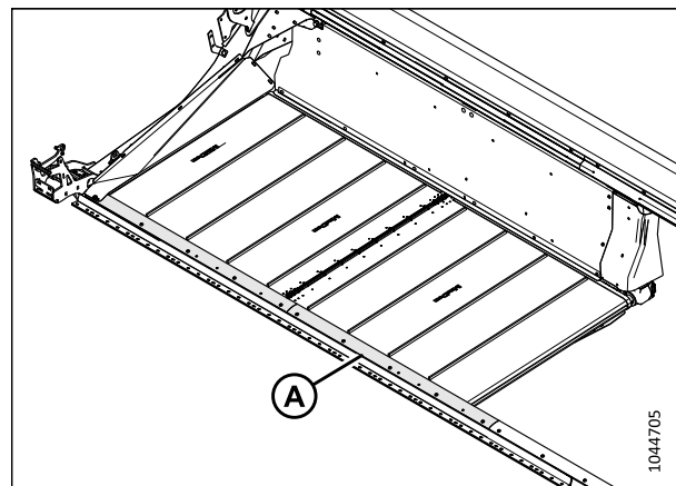
Figure 5.95: Joints de barre de coupe
