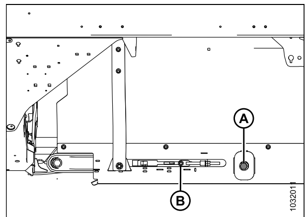
Figure 5.113: Tendeur de tapis
