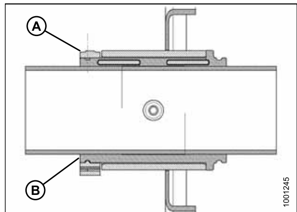
Figure 5.168: Bague
