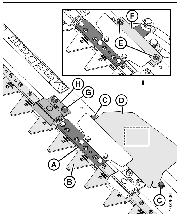
Figure 5.238: Couteau vertical – Protection enlevée
