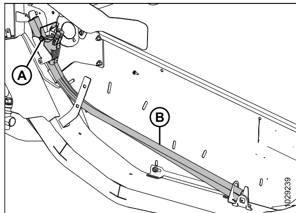
Figure 3.80: Tiges de division
