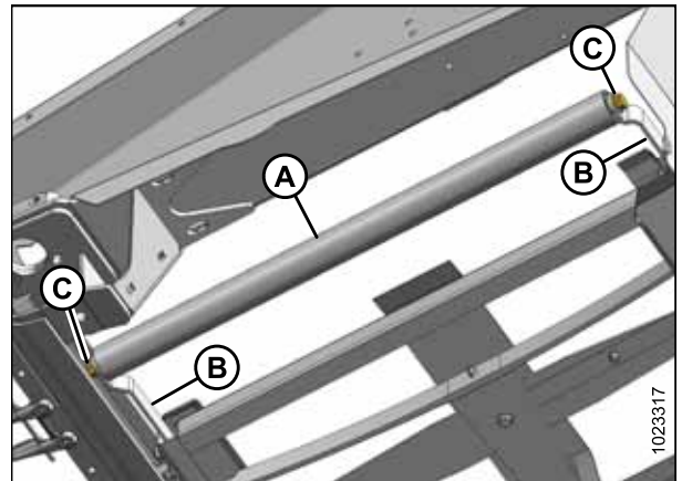
Figure 5.110: Rouleau libre
