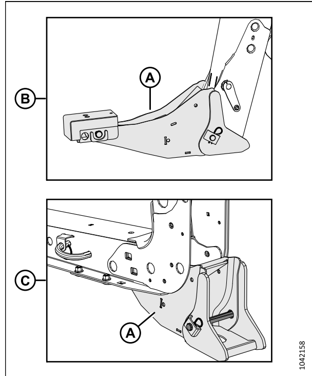
Figure 4.125: Supports de la plateforme installés
