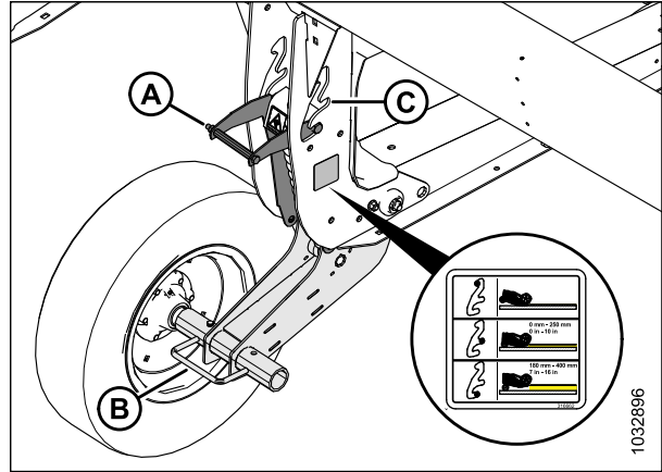
Figure 3.33: Roue stabilisatrice
