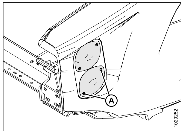
Figure 5.19: Option transport – feux oranges et rouges
