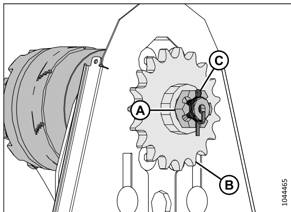
Figure 5.214: Pignon unique
