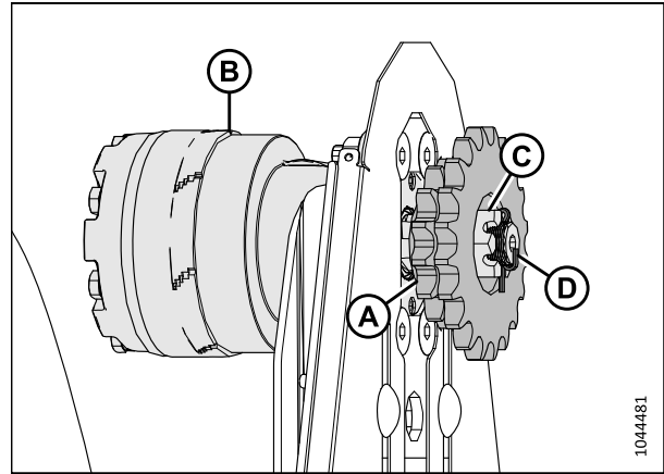
Figure 5.220: Pignon double
