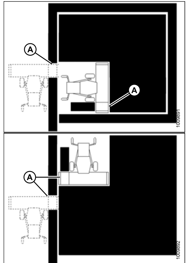
Figure 3.93: Double andainage
