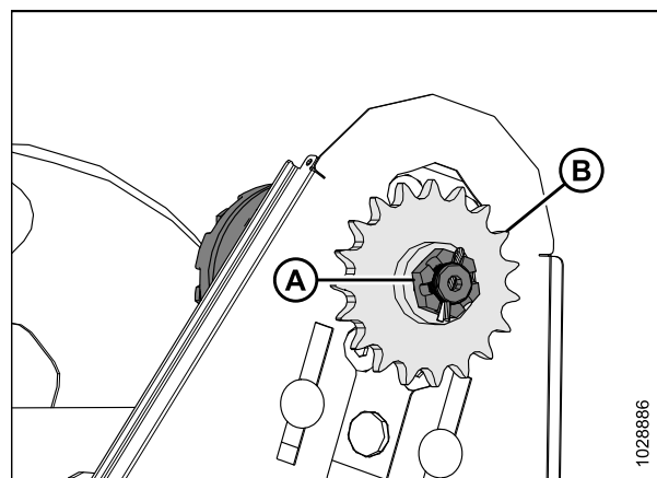
Figure 5.213: Pignon unique
