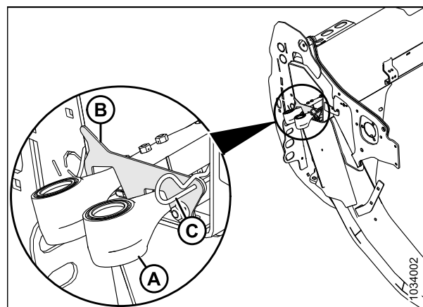
Figure 5.41: Couteaux de rechange
