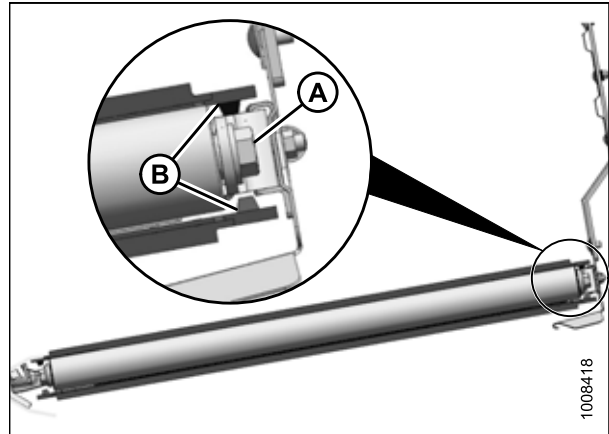
Figure 5.98: Rouleau libre
