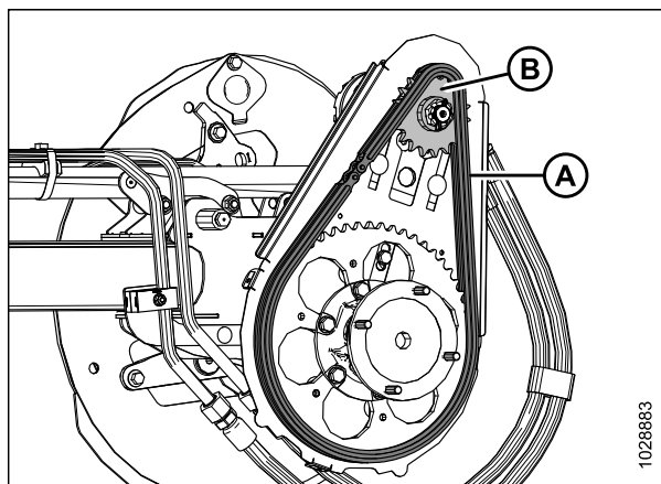
Figure 5.215: Pignon unique
