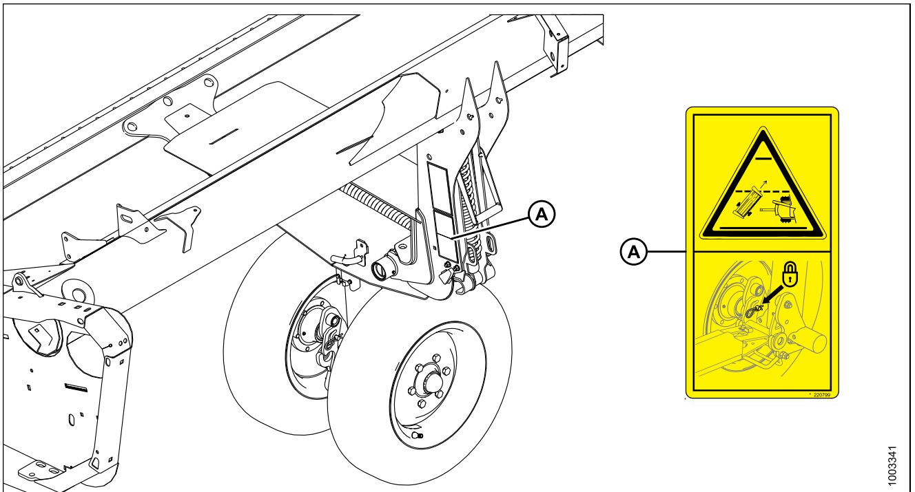
Figure 1.29: Option de transport EasyMove MC (facultative)
