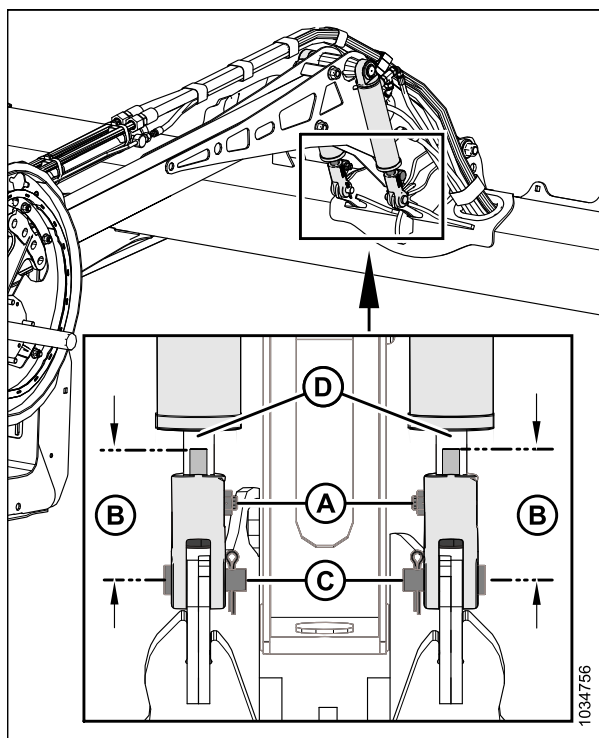
Figure 5.140: Cylindres du bras central
