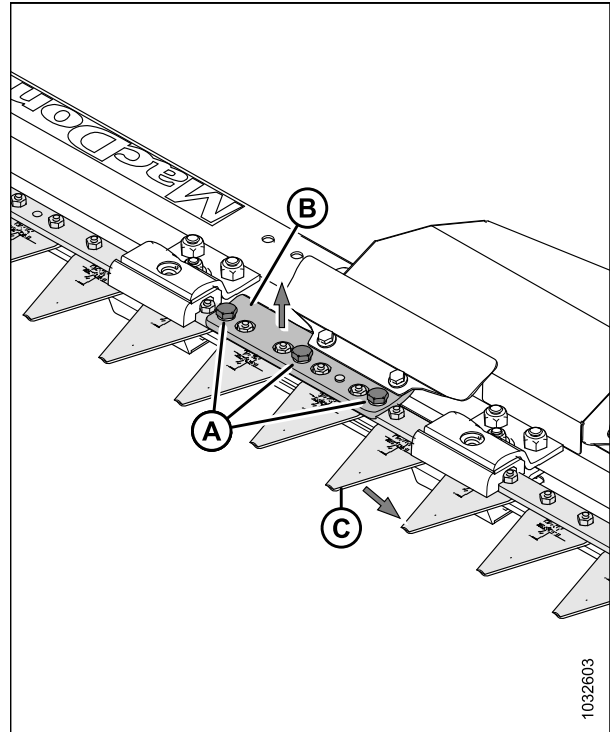
Figure 5.237: Couteau vertical – Protection enlevée
