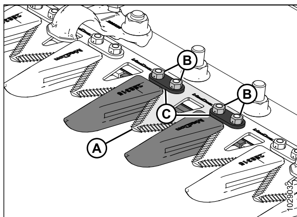
Figure 5.32: Barre de coupe
