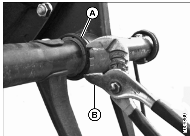
Figure 5.181: Installation du collier
