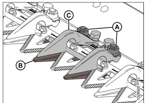
Figure 5.69: Doigts de couteau court
