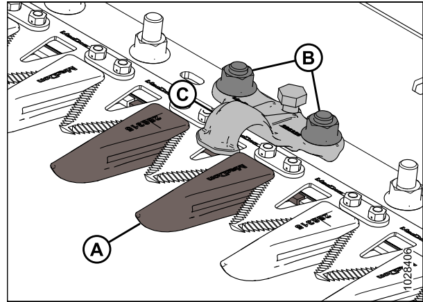
Figure 5.52: Doigts de couteau pointus
