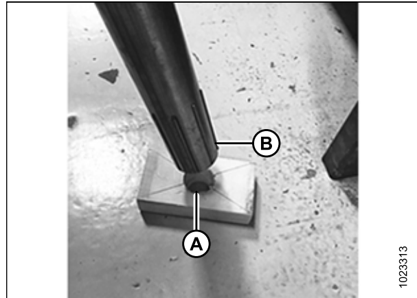
Figure 5.107: Rouleau libre
