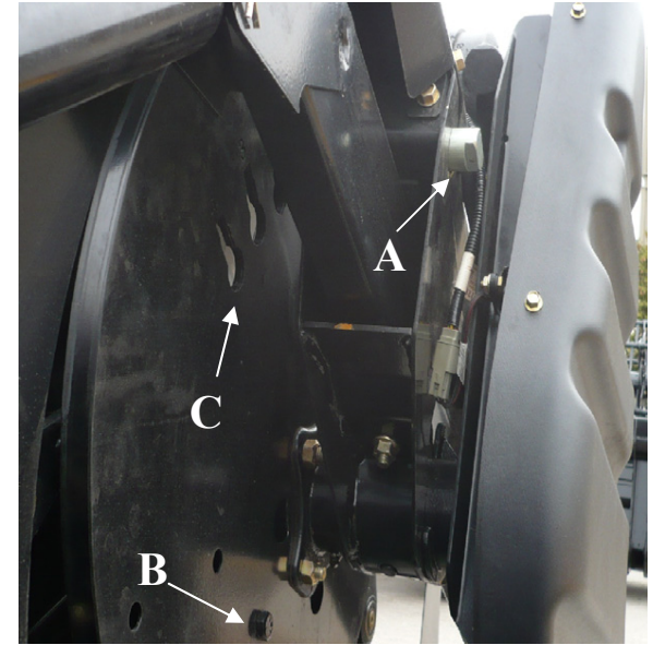
Figure 2 Reel Tine Pitch Adjustment
