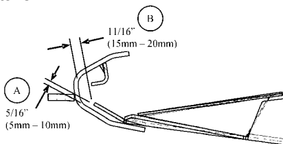
PAN CLEARANCE TO CUTTERBAR 972/973/974 HEADER
