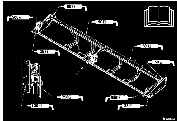
DOUBLE KNIFE
