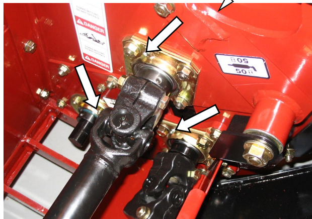
ROLL SHAFT BEARINGS (3 PLCS)
