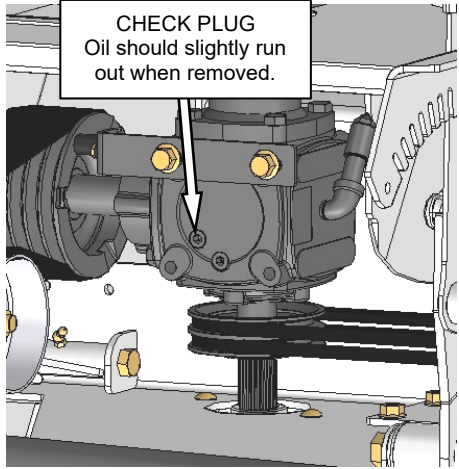
GEARBOX OIL LEVEL
