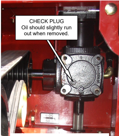
GEARBOX OIL LEVEL
