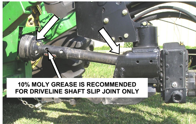
PTO DRIVELINE
