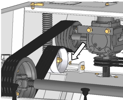
BELT TENSIONER PIVOT (1 PLC)
