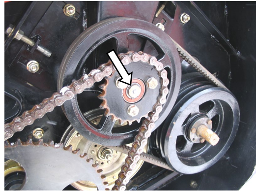
AUGER DRIVE BEARING (1 PLC)
