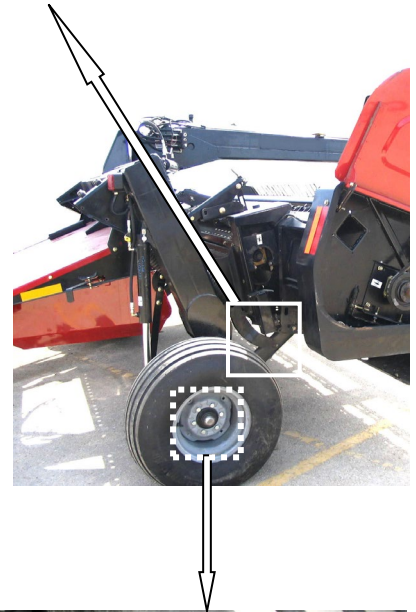
FLOAT LINK (3 PLCS) BOTH SIDES
