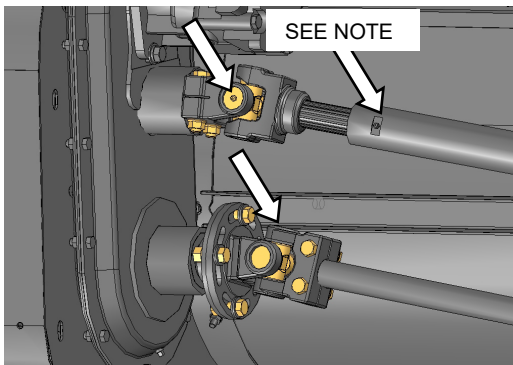
DRIVELINE UNIVERSALS (2 PLCS) DRIVELINE SHAFTS (1 PLC)
