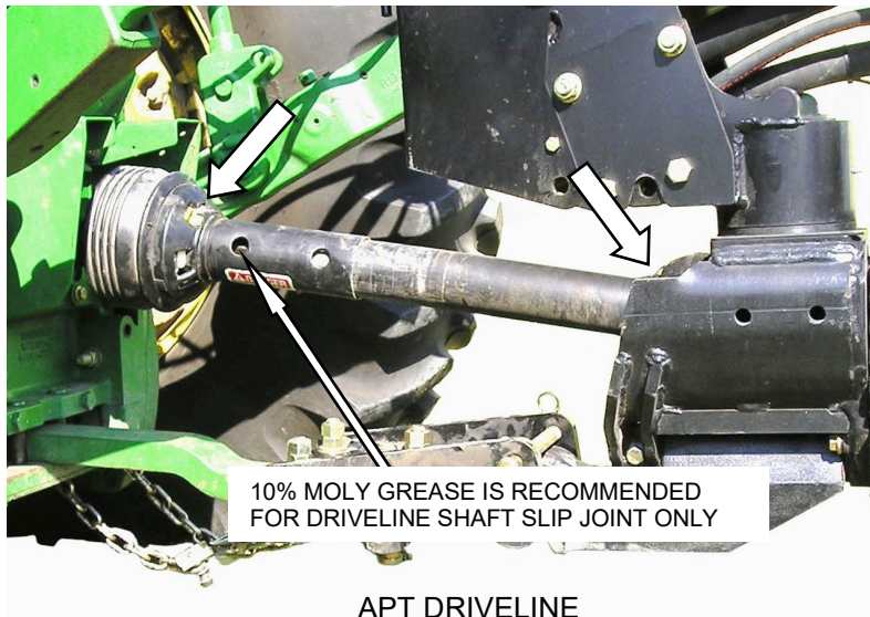
APT DRIVELINE
